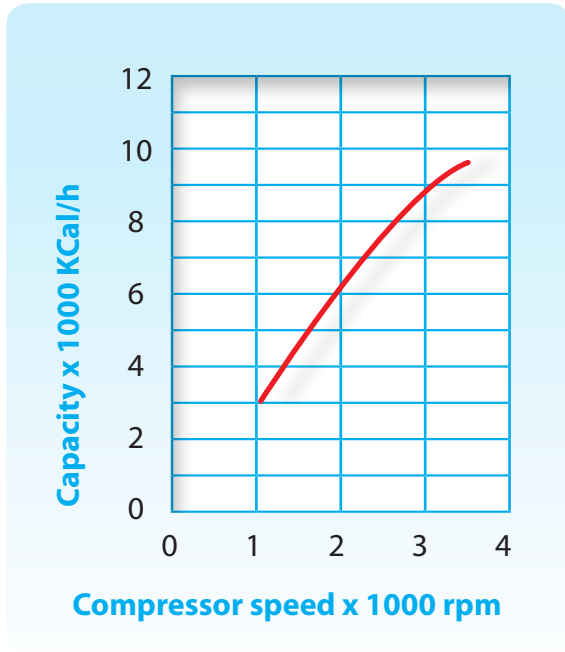
Graph 7. Compressor 2 performance
