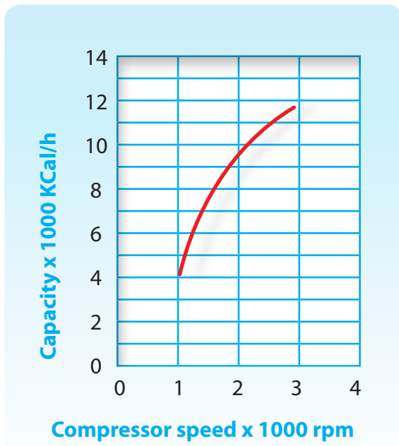
Graph 7. Compressor 2 performance
