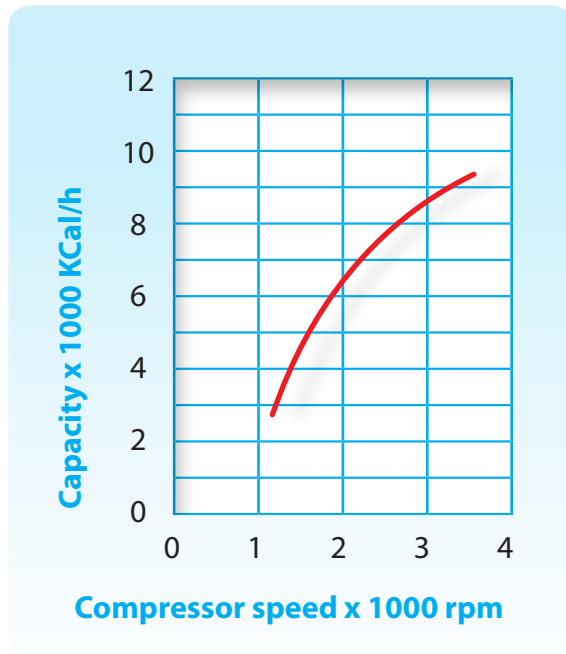
Graph 5. Compressor performance 2
